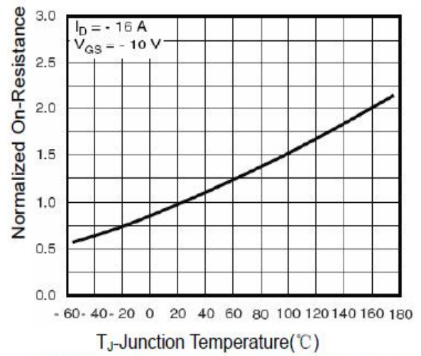
Figure 4 Rdson-Junction Temperature
