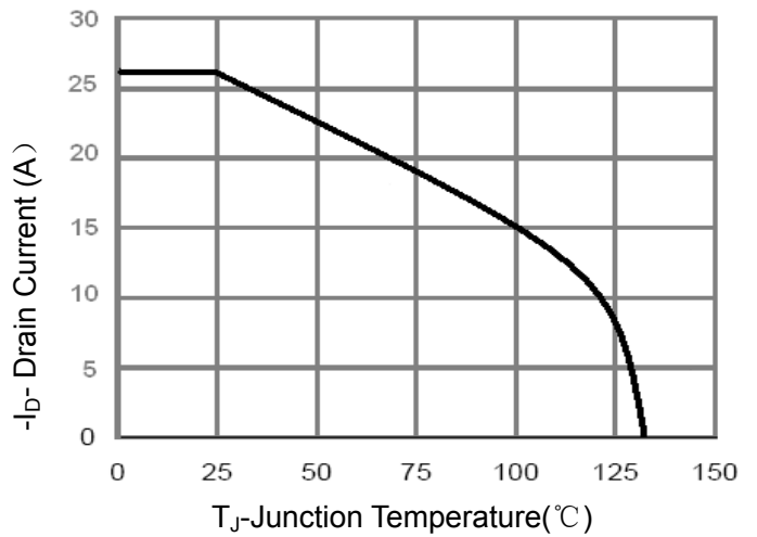
Figure 4 Drain Current
