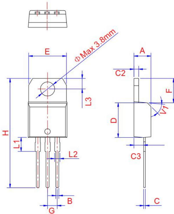
TO-220B Non-Ins
