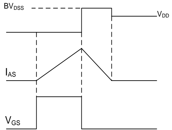
Fig.10 EAS Waveform
