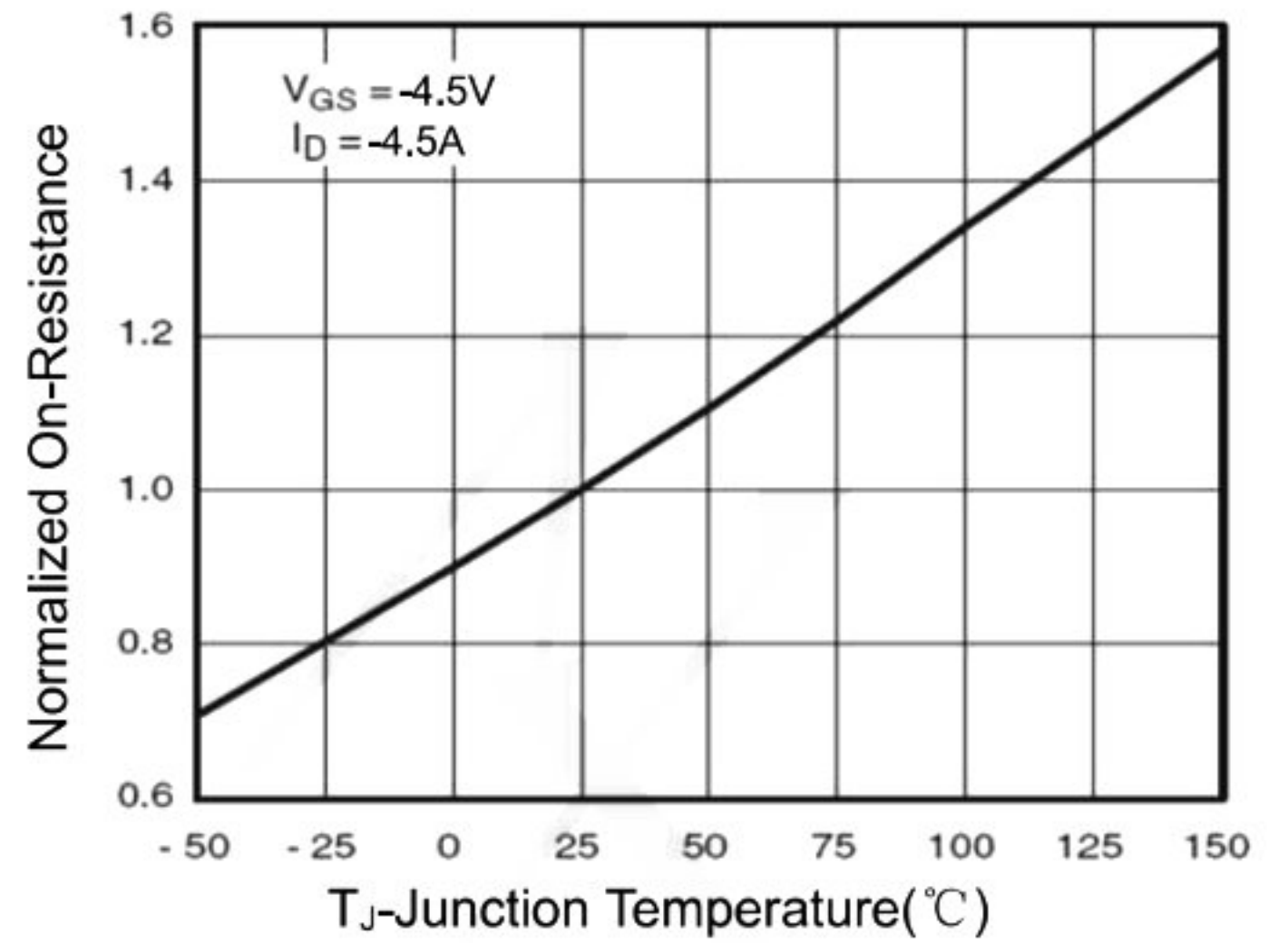
Figure 8 Drain-Source On-Resistance
