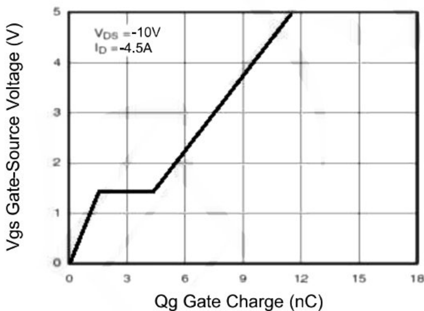
Figure 11 Gate Charge
