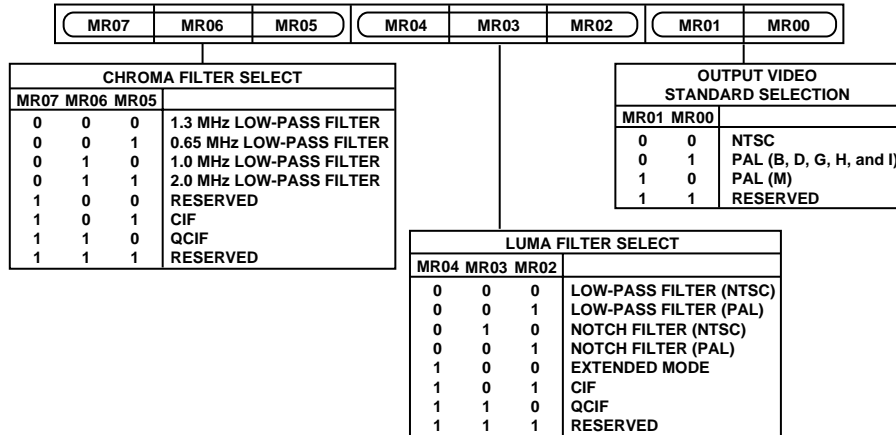
Figure 38. Mode Register 0
