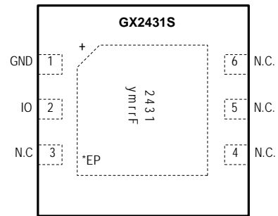
DFN (4mm x 4mm)
