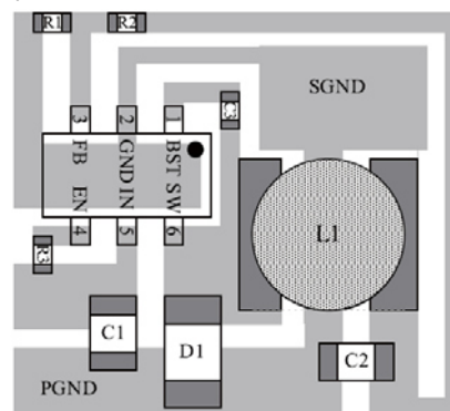
Figure 2: PCB Layout
