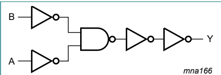
Fig. 3. Logic diagram
