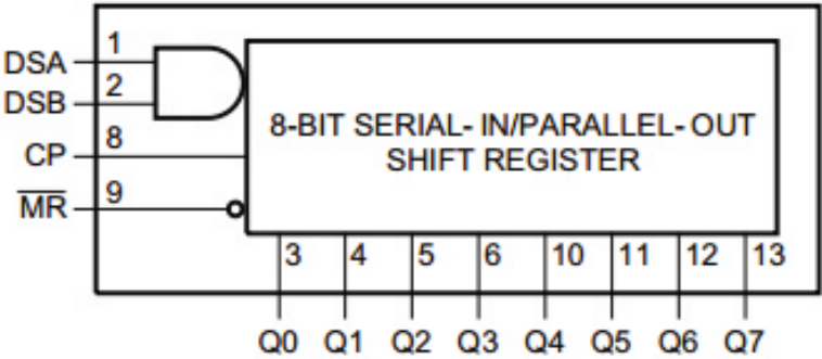
Figure 3. Logic diagram
