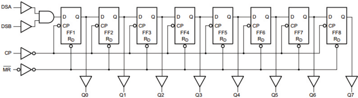
Figure 4. Functional diagram
