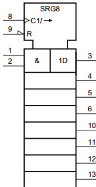
Figure 2. IEC logic symbol
