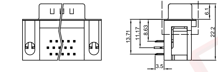
With screw and rivet type
