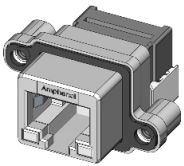
MRJ-5480-01 Rugged RJ45, 8 Position, Vertical
