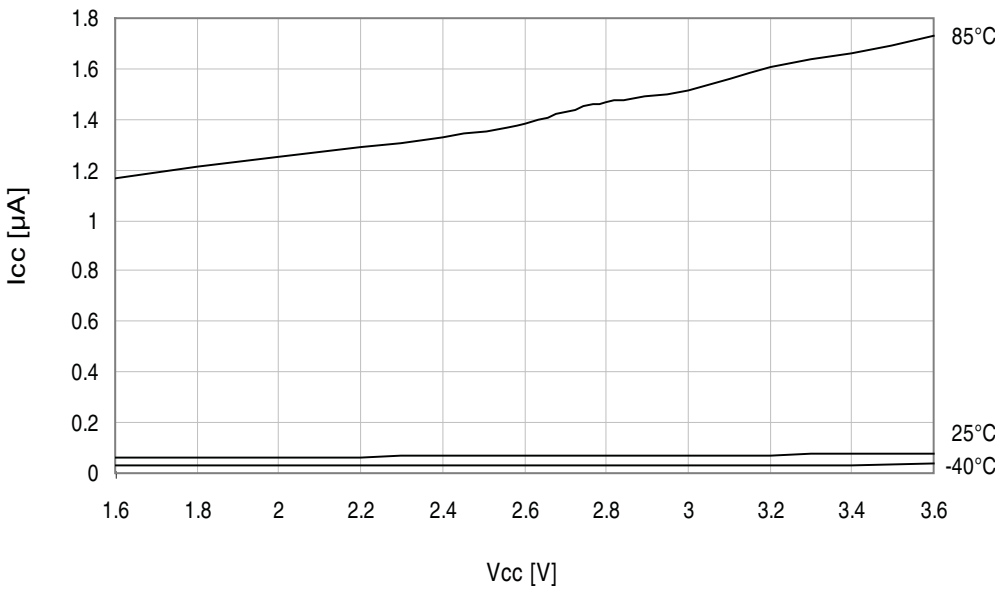
Figure 33-256. Power-down mode supply current vs. V_{CC} . All functions disabled.
