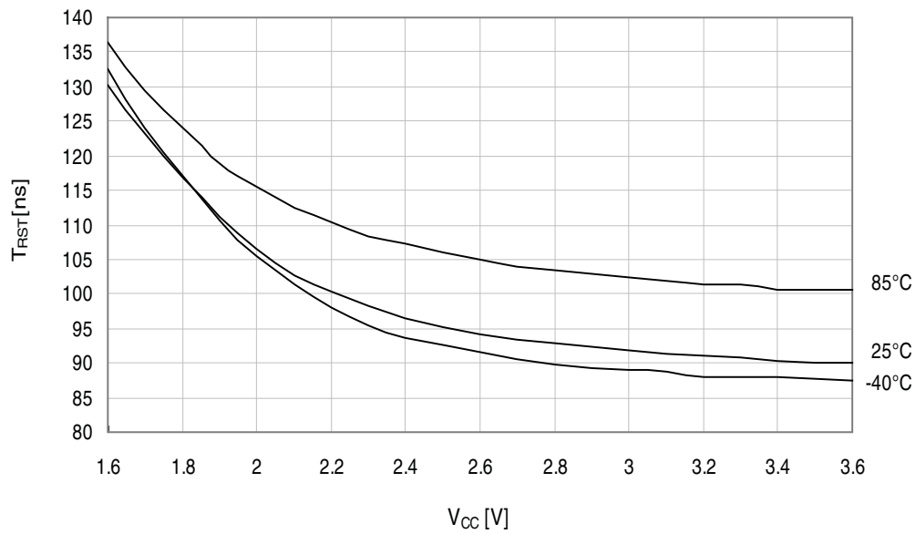
Figure 33-57. Minimum Reset pin pulse width vs. V_{CC} .
