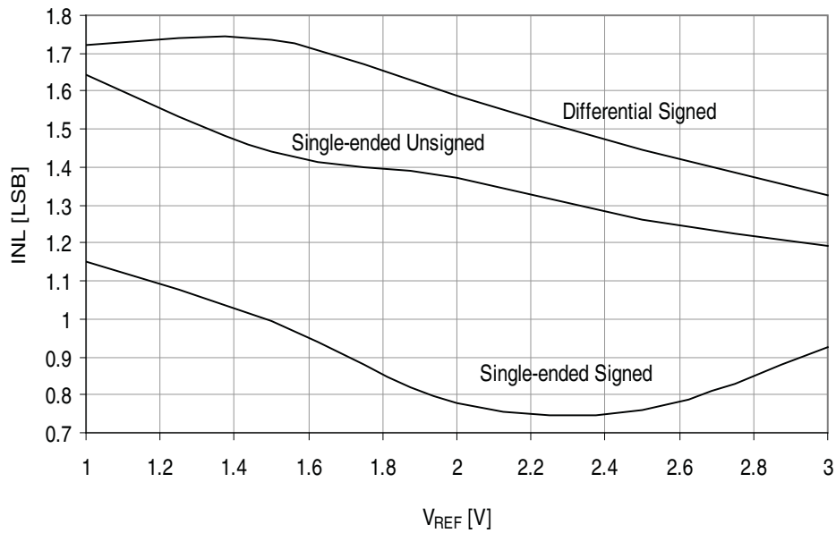
Figure 33-276. INL error vs. external V_{REF} .
