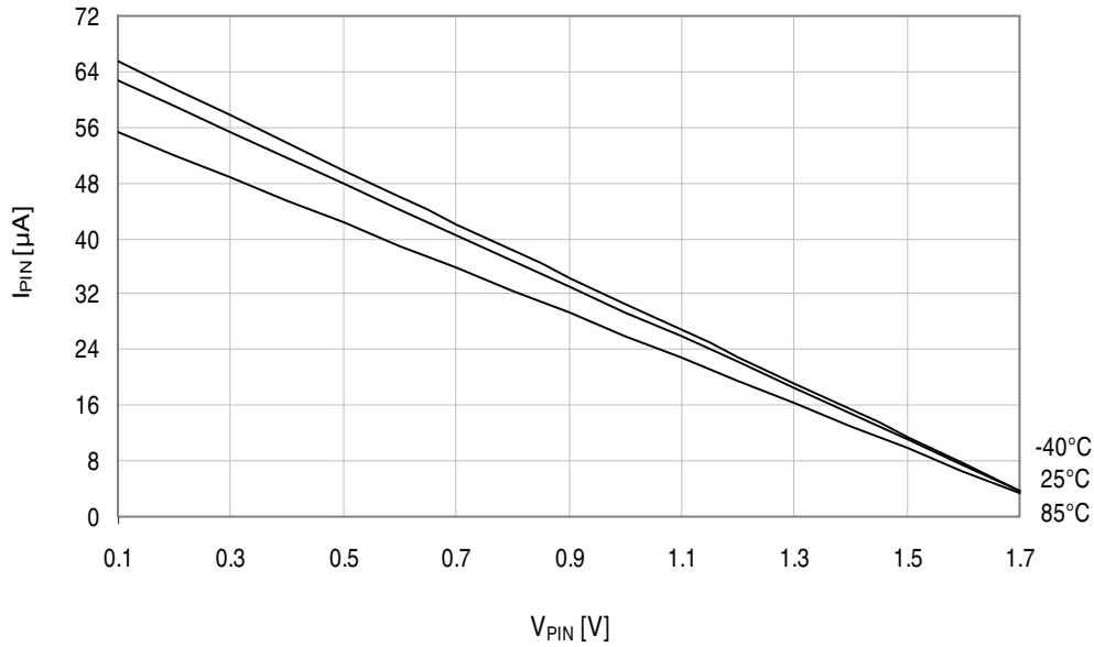
Figure 33-101. I/O pin pull-up resistor current vs. input voltage.
