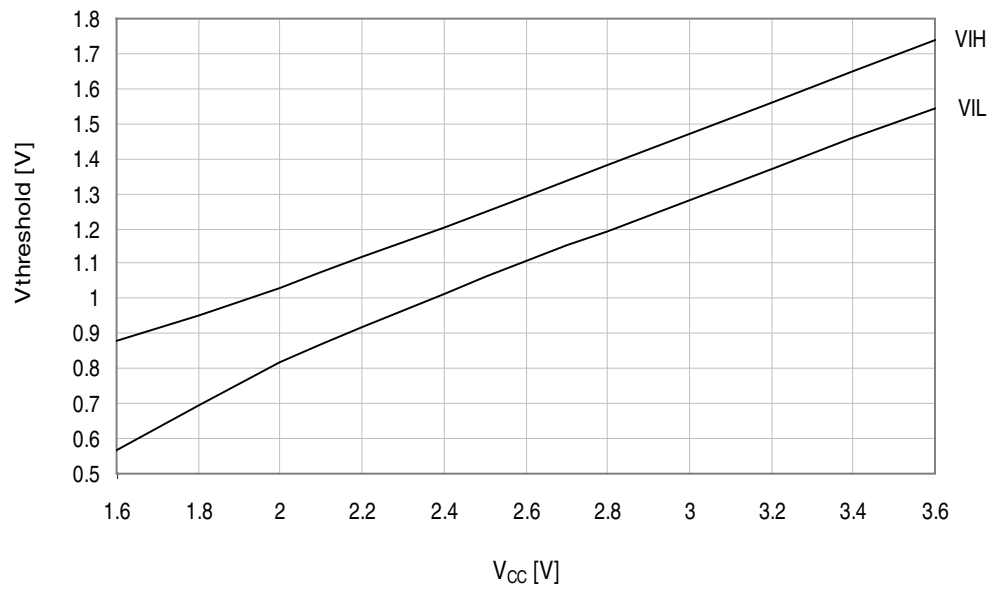
Figure 33-32. I/O pin input threshold voltage vs. V_{CC} .
