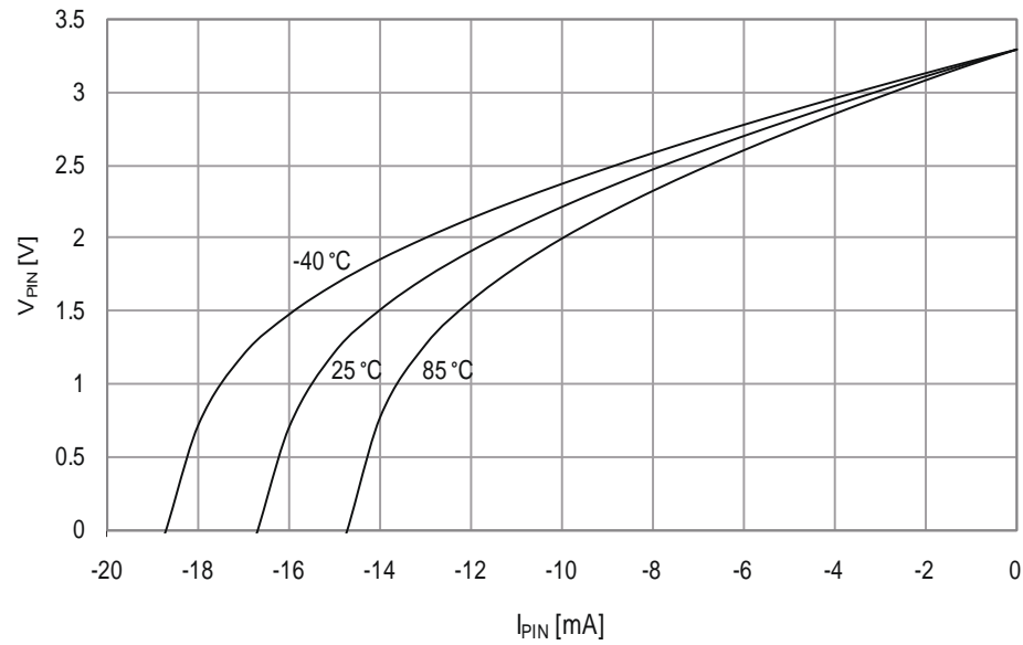
Figure 34-24. I/O pin output voltage vs. source current.
