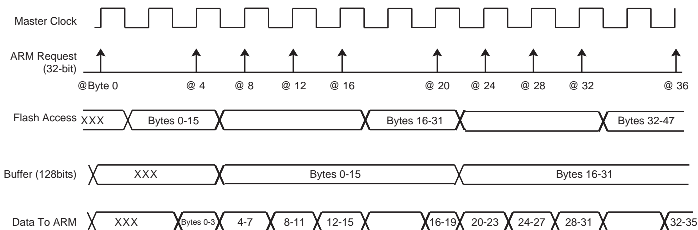
Figure 20-4. Data Read Optimization for FWS = 1
