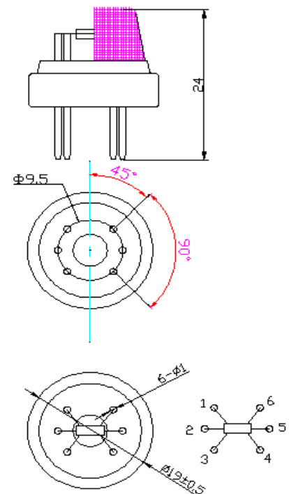
Fig1.Sensor Structure
