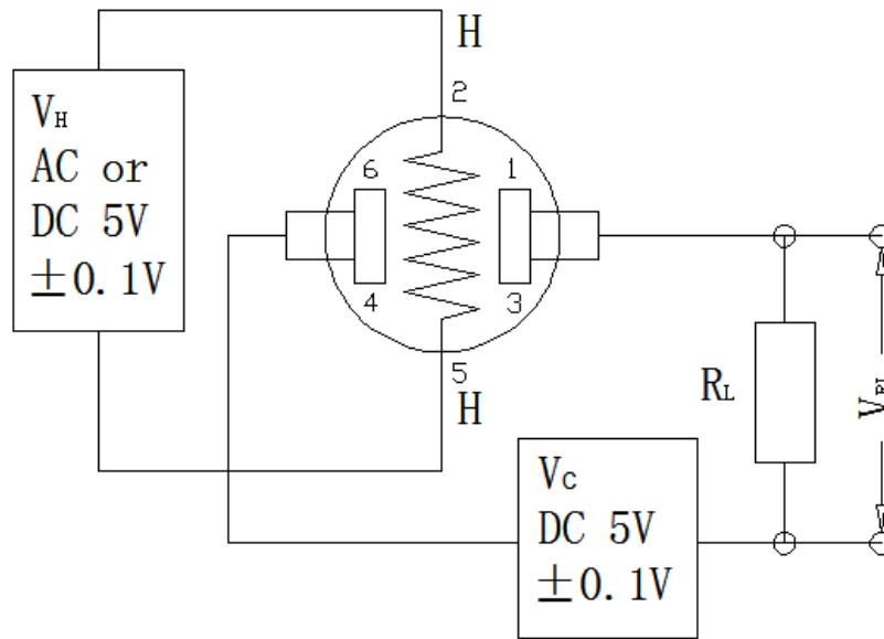
Fig2. GQ-131a HC HC Test Circuit
