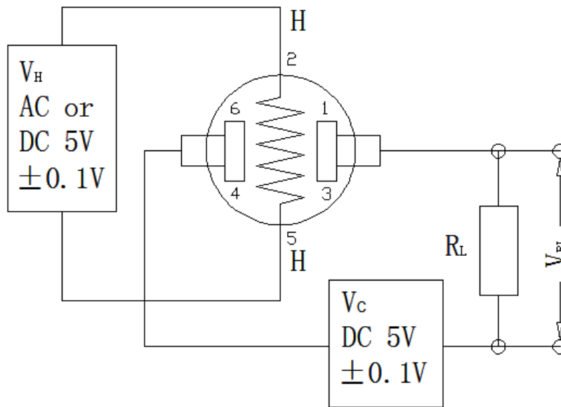
Fig2. GQ-131a LC Test Circuit
