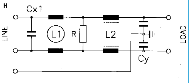
Circuit diagram
