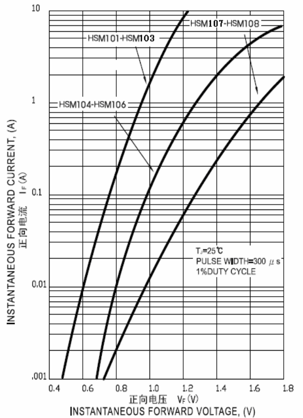
FIG. 4- 瞬間正向特性曲線(典型值) FIG. 4 - TYPICAL INSTANTANEOUS FORWARD CHARACTERISTICS
