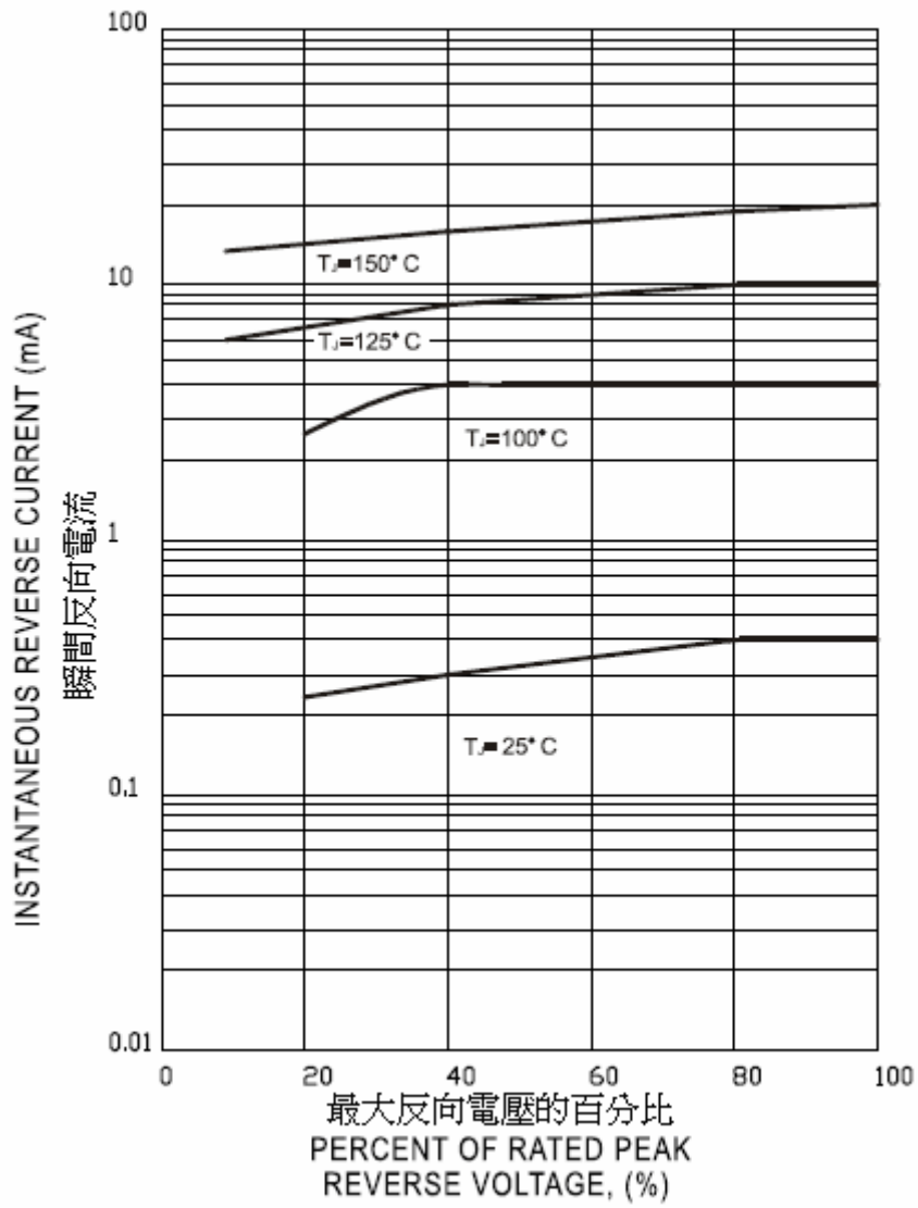
FIG. 5 – TYPICAL REVERSE CHARACTERISTICS
