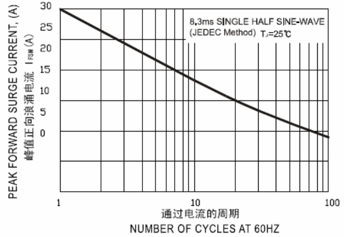
FIG. 2- 浪涌特性曲線 (最大值) FIG. 2 - MAXIMUM NON-REPETITIVE PEAK FORWARD SURGE CURRENT
