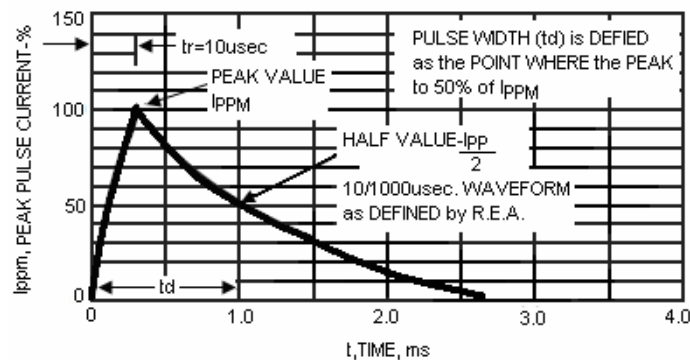
FIG.3-PULSE WAVEFORM
