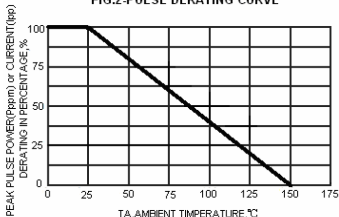
FIG.2-PULSE DERATING CURVE
