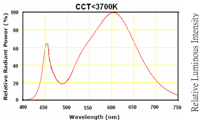
Fig.3 Wavelength Characteristics(Ta=25°C)
