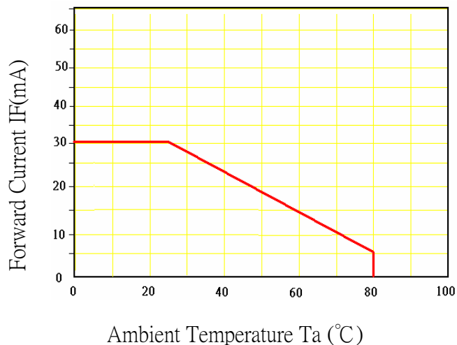
Fig.5 IF-Ta
