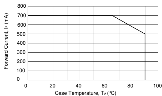
<Fig.a> Forward Current Derating Curve
