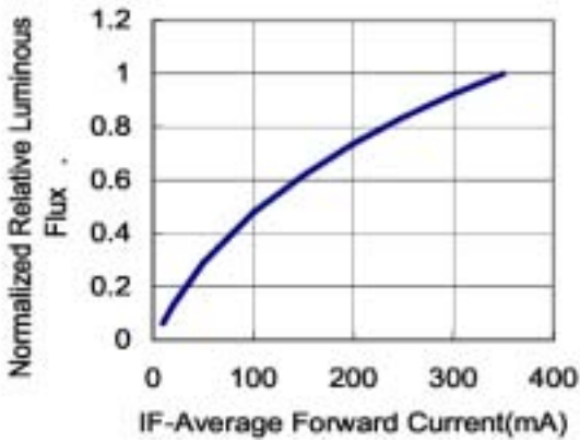
Fig 4a. Relative Luminous Flux vs. Forward Current for White, Blue and Green at T_j=25 maintained.
