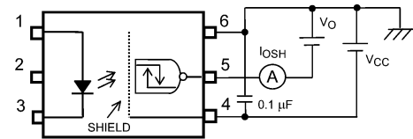
Fig. 12.1.6 IOSH Test Circuit
