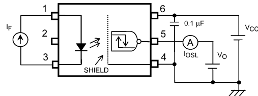
Fig. 12.1.5 IOSL Test Circuit
