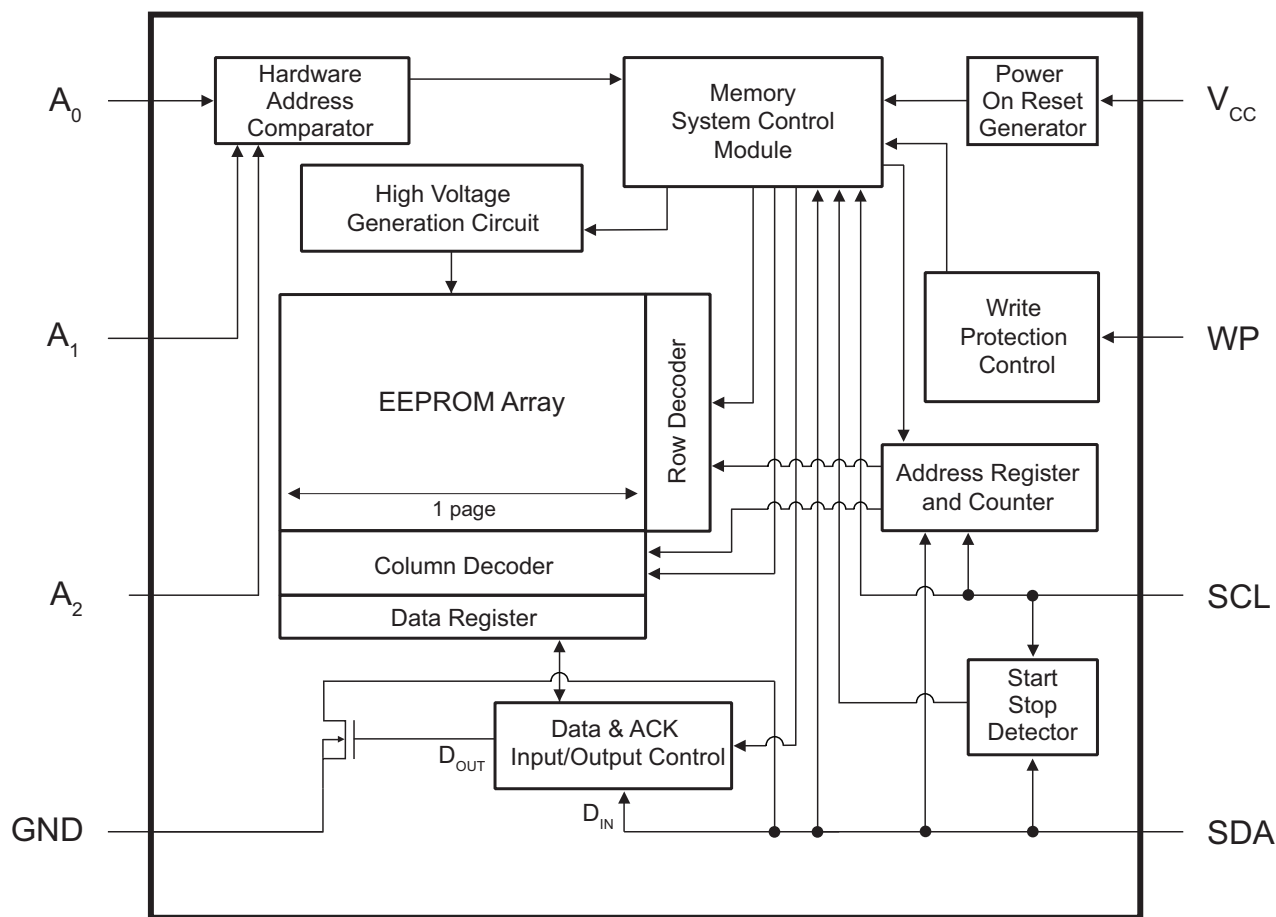
Figure 2-1. Block Diagram
