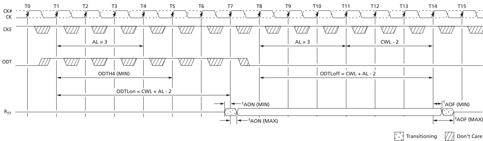
Figure 113: Synchronous ODT
