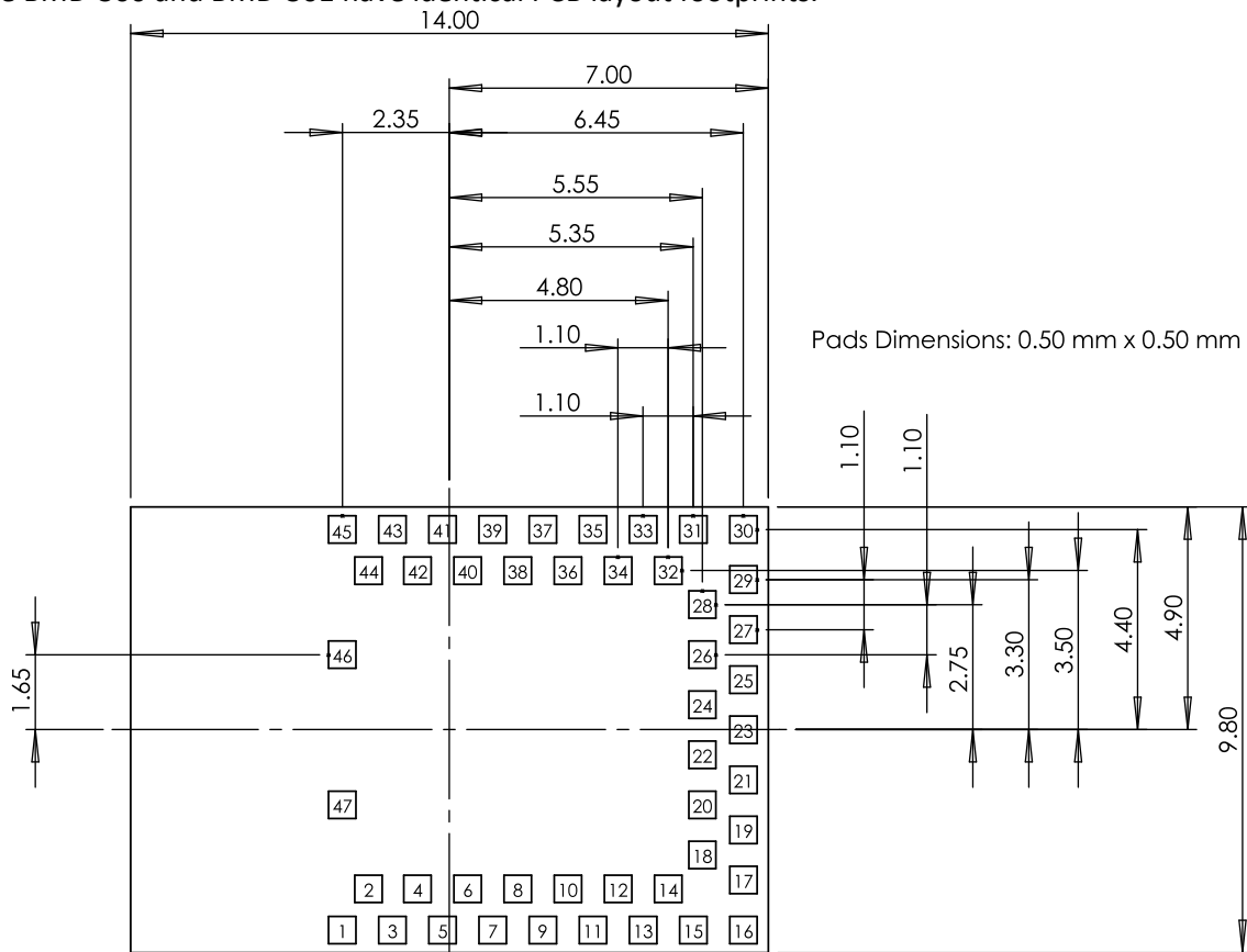
Figure 8 – BMD-300/301 Dimensions (Top View)
