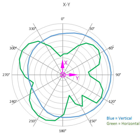
Figure 16 – X-Y Plane Antenna Pattern
