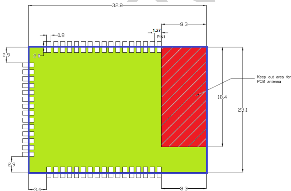
Figure 4. HF-LPB100 PCB Symbol Size
