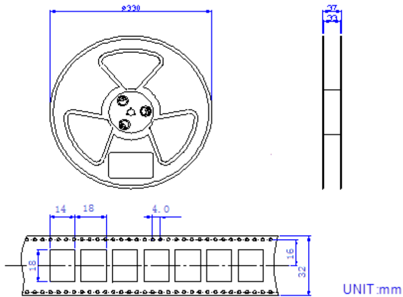
Figure 6: SKB360 Packaging
