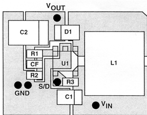
FIGURE 1. Recommended PCB Component Layout
