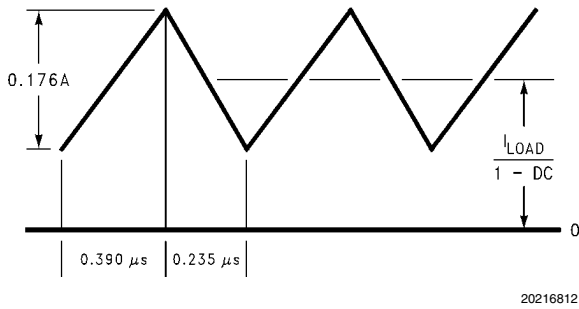
FIGURE 2. 10 μH Inductor Current, 5V–12V Boost
