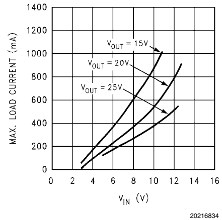
FIGURE 4. Max. Load Current vs V_IN
