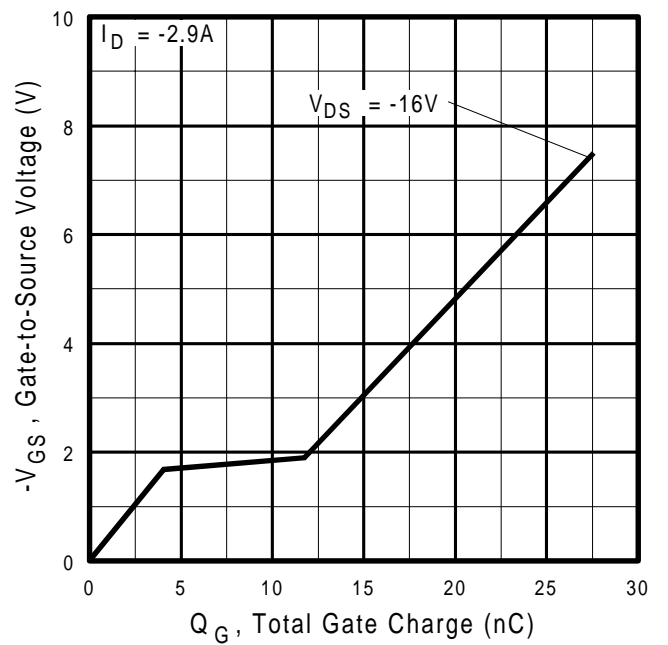
Fig 10. Typical Gate Charge Vs. Gate-to-Source Voltage
