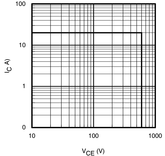
Fig. 4 - Reverse Bias SOA T_J = 175^{\circ}C ; V_{CE} = 15V
