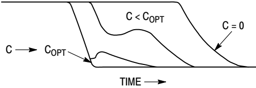
Figure 8. Turn-Off Waveform
