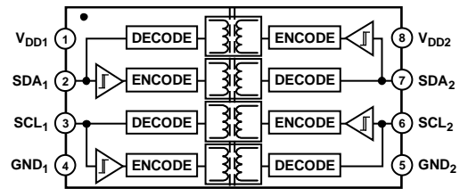
Figure 1. ADuM1250
