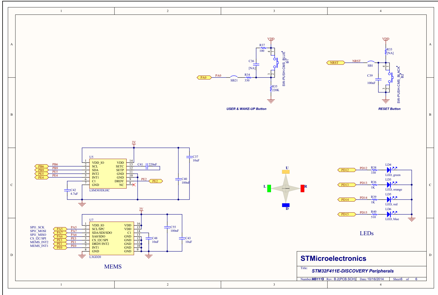
Figure 14. Peripherals
