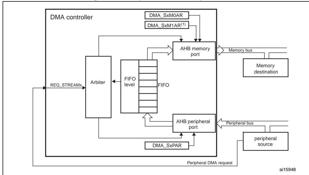
Figure 36. Peripheral-to-memory mode
