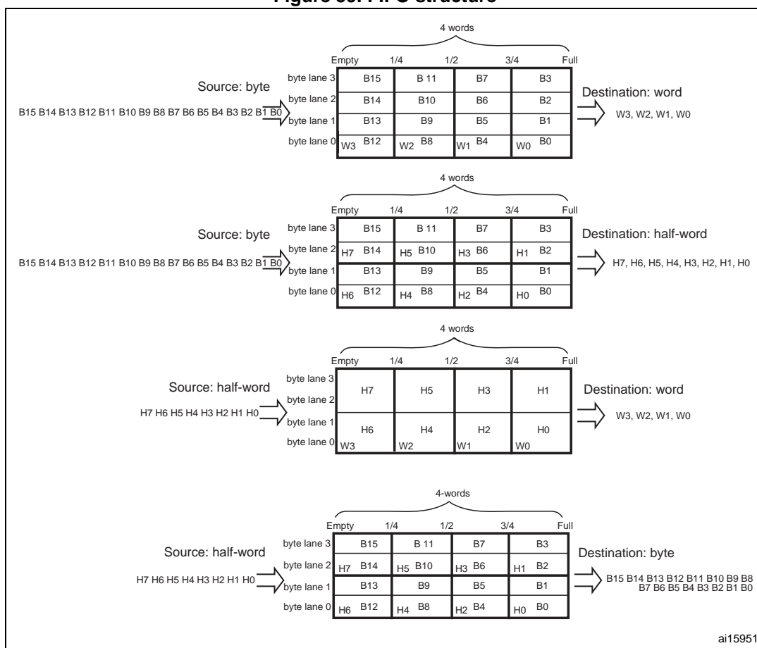
Figure 39. FIFO structure
