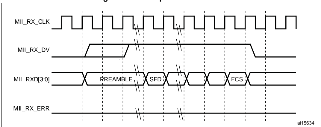
Figure 367. Reception with no error
