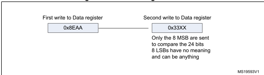
Figure 266. Transmitting 0x8EAA33
