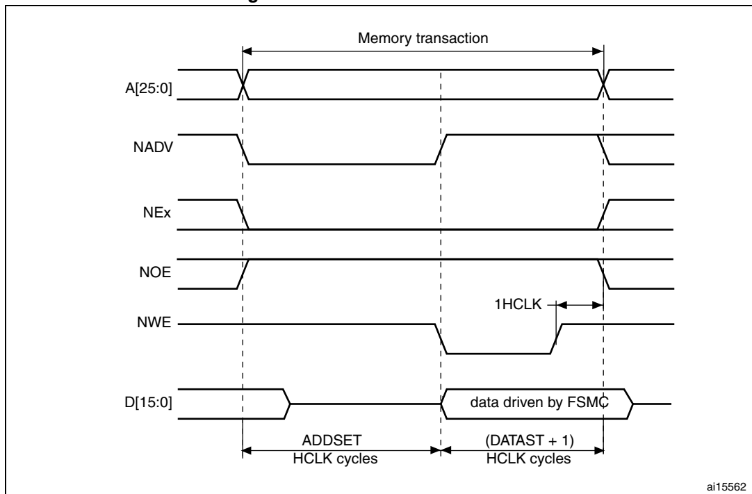
Figure 440. Mode B write accesses
