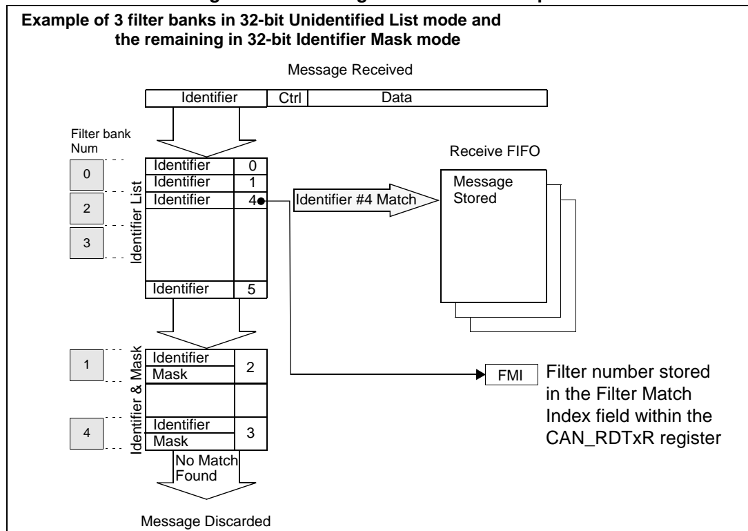
Figure 344. Filtering mechanism - example
