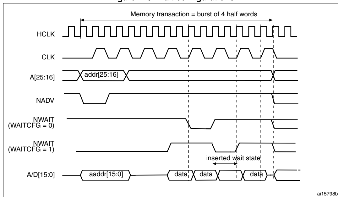
Figure 449. Wait configurations
