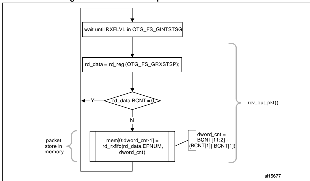
Figure 424. Receive FIFO packet read in slave mode
