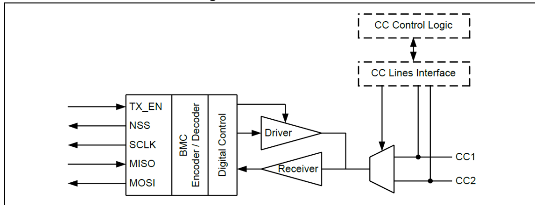
Figure 3. BMC interface
