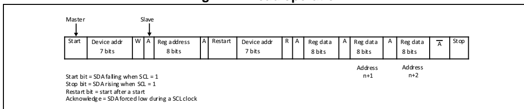
Figure 5. Read operation
