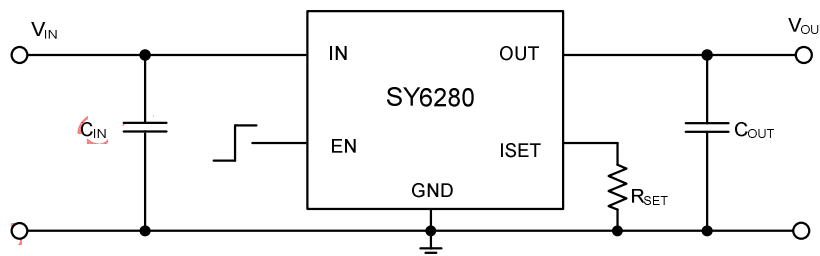
Figure 1. Schematic Diagram
