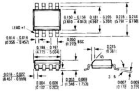
8 Lead Small Outline \theta_{JA} = 170\text{ C/W} \theta_{JC} = 80\text{ C/W}
