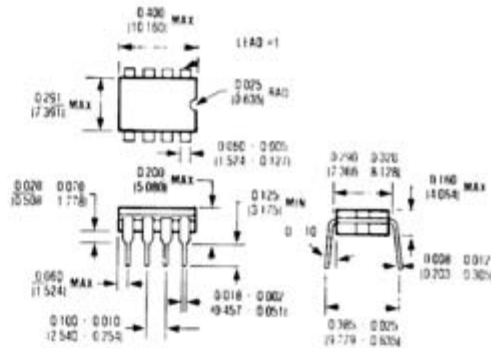
8 Lead Cerdip \theta_{JA} = 125\text{ C/W} \theta_{JC} = 55\text{ C/W}
