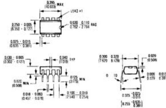
8 Lead Plastic DIP \theta_{JA} = 120\text{ C/W} \theta_{JC} = 70\text{ C/W}
