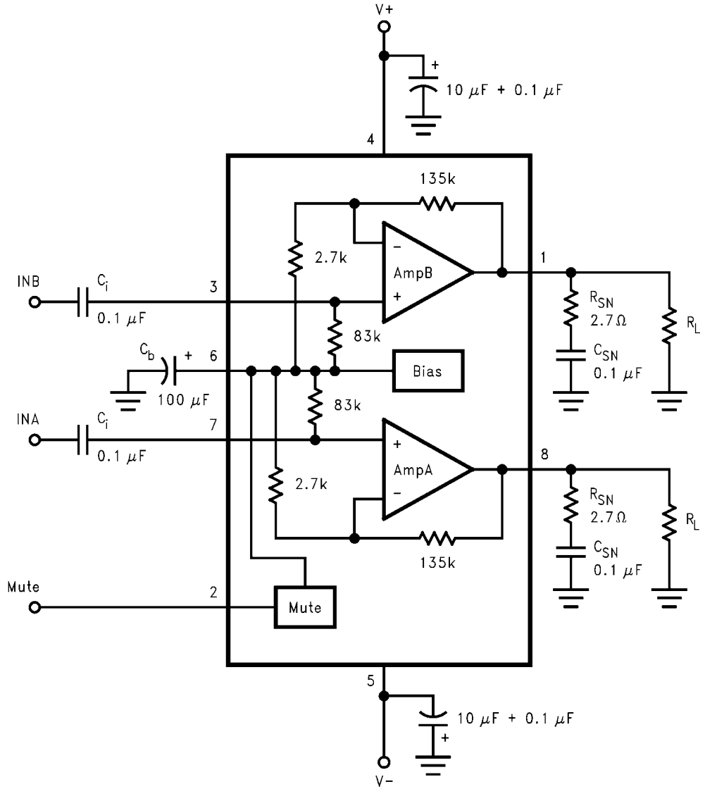
FIGURE 2. Test Circuit
