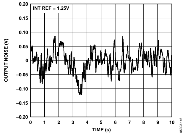
Figure 46. 0.1 Hz to 10 Hz Output Noise Plot, Internal Reference
