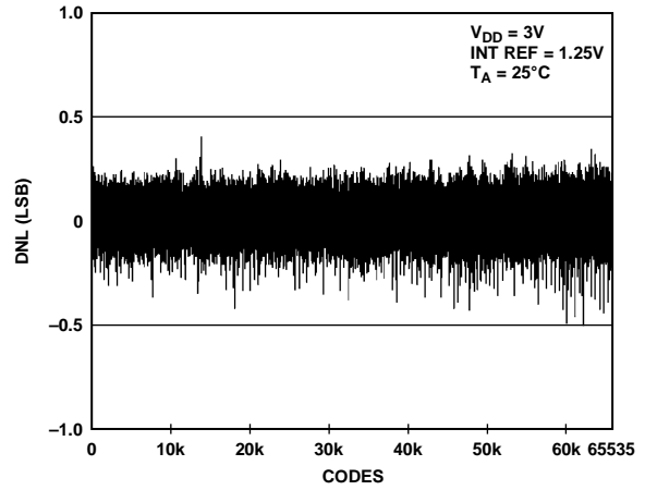
Figure 21. DNL AD5668-1
