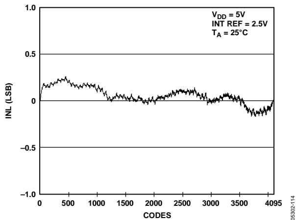
Figure 14. INL AD5628-2
