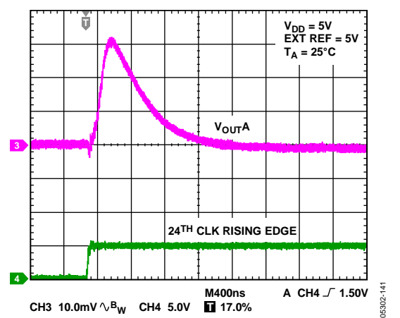
Figure 41. Digital-to-Analog Glitch Impulse (Negative)
