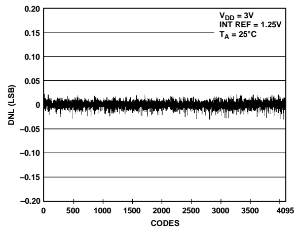
Figure 23. DNL AD5628-1
