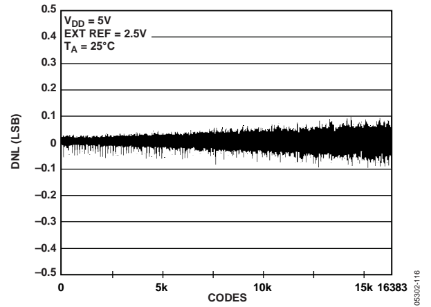
Figure 16. DNL AD5648-2
