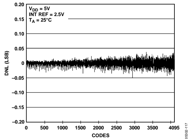
Figure 17. DNL AD5628-2
