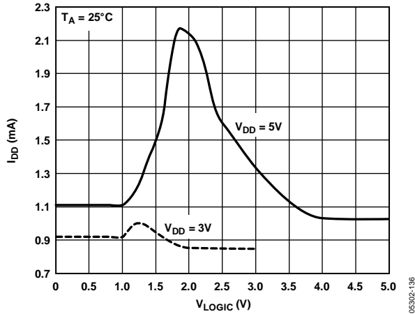
Figure 36. Supply Current vs. Logic Input Voltage
