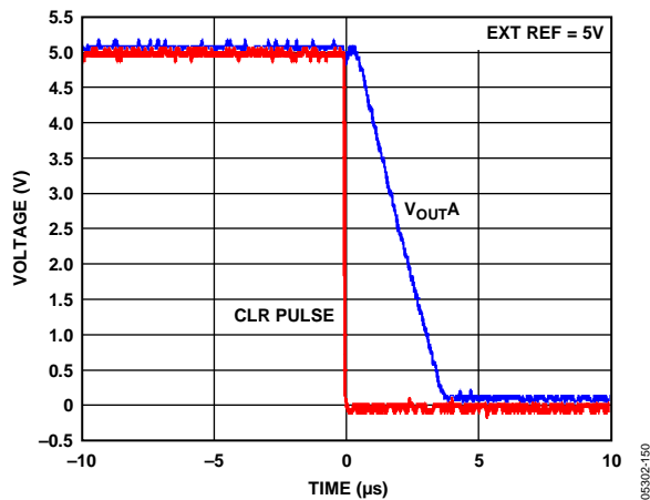
Figure 50. Hardware \overline{\text{CLR}}
