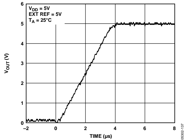
Figure 37. Full-Scale Settling Time, 5 V
