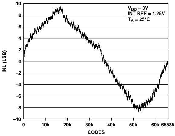
Figure 18. INL AD5668-1
