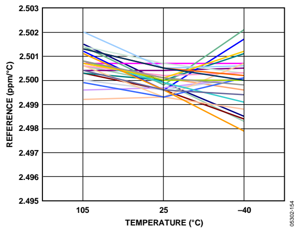
Figure 53. 2.5 V Reference Temperature Coefficient vs. Temperature
