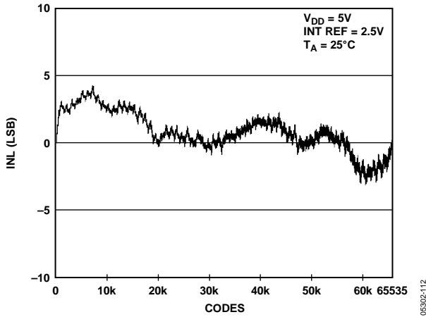
Figure 12. INL AD5668-2/AD5668-3
