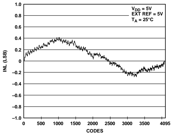
Figure 8. INL AD5628—External Reference
