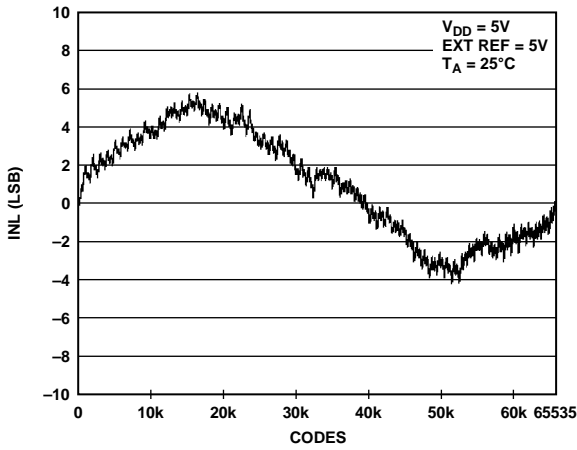
Figure 6. INL AD5668—External Reference
