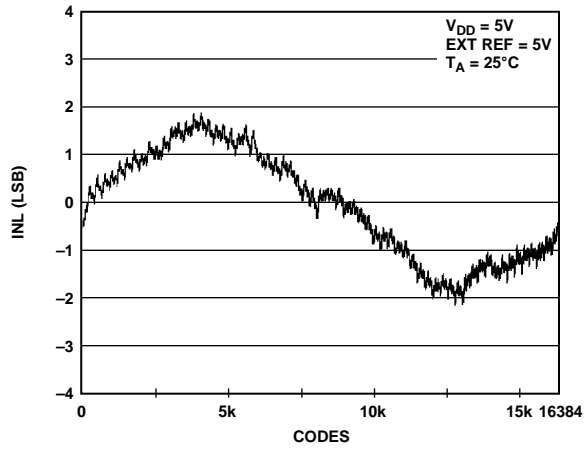
Figure 7. INL AD5648—External Reference
