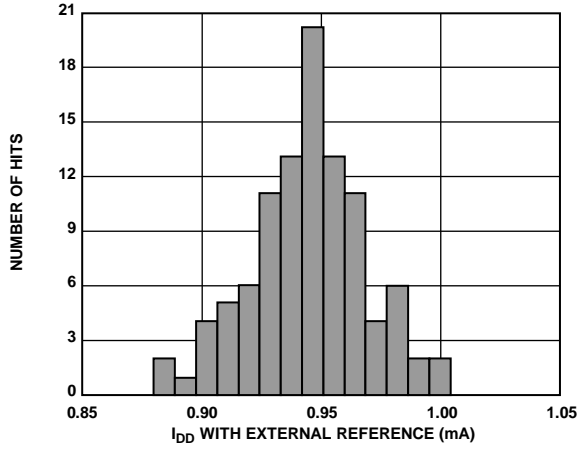
Figure 28. I_{DD} Histogram with External Reference
