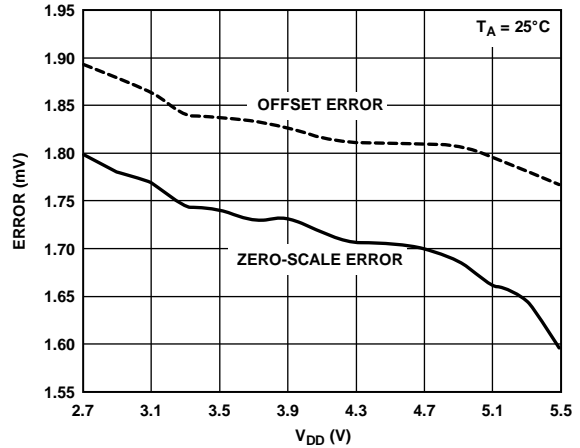
Figure 27. Zero-Scale Error and Offset Error vs. Supply Voltage
