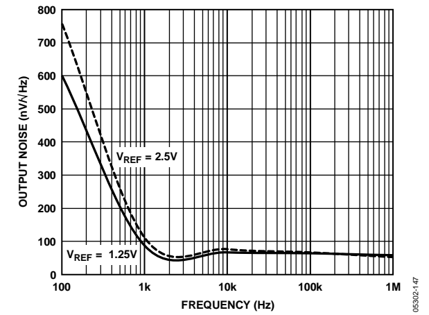
Figure 47. Noise Spectral Density, Internal Reference
