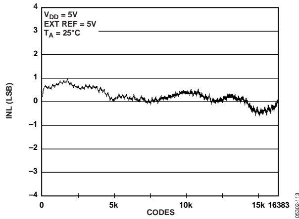
Figure 13. INL AD5648-2
