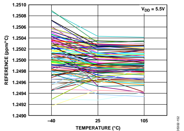
Figure 52. 1.25 V Reference Temperature Coefficient vs. Temperature
