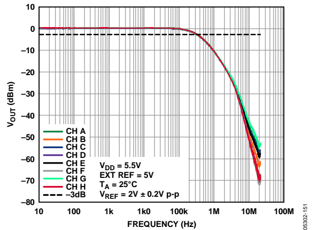
Figure 51. Multiplying Bandwidth
