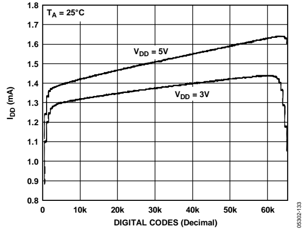
Figure 33. Supply Current vs. Code
