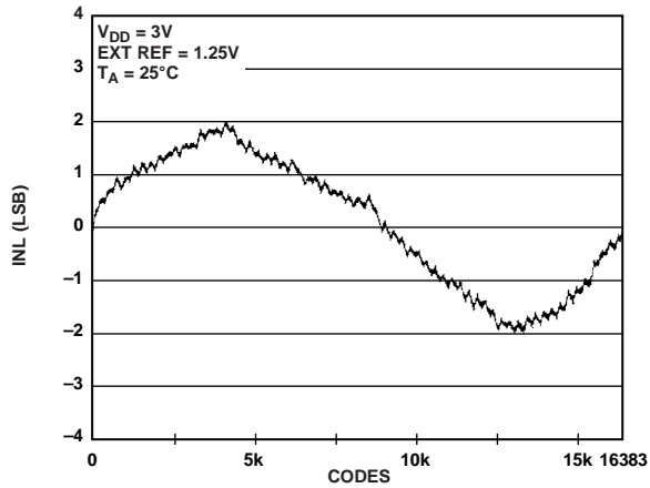
Figure 19. INL AD5648-1
