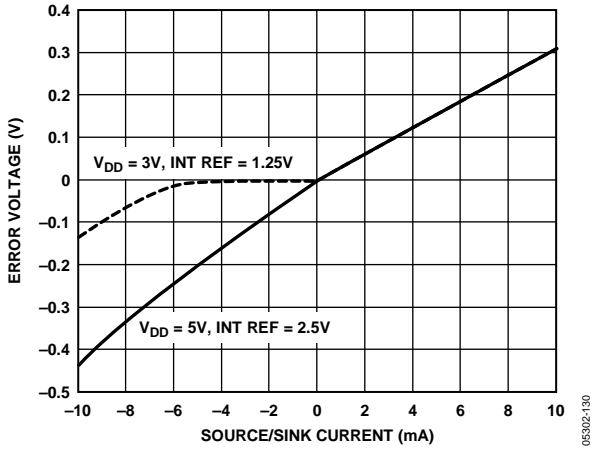
Figure 30. Headroom at Rails vs. Source and Sink
