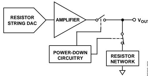
Figure 60. Output Stage During Power-Down
