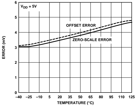
Figure 25. Zero-Scale Error and Offset Error vs. Temperature
