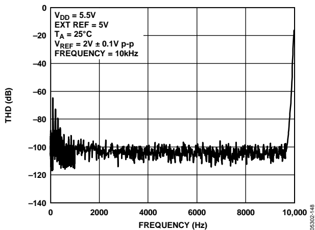
Figure 48. Total Harmonic Distortion
