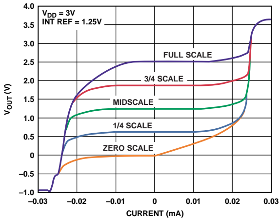
Figure 32. AD5668-1 Source and Sink Capability
