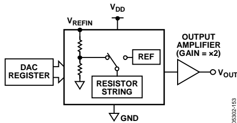
Figure 54. DAC Architecture
