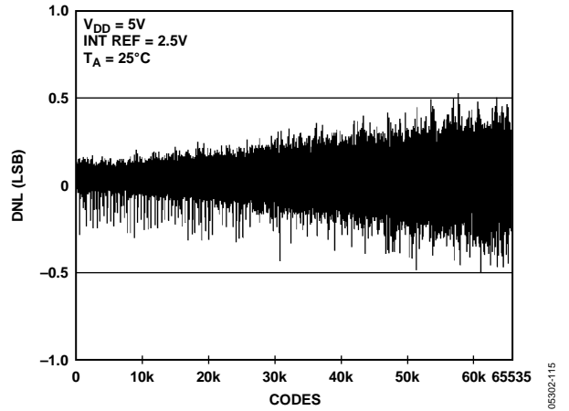
Figure 15. DNL AD5668-2/AD5668-3
