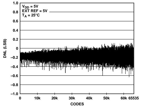
Figure 9. DNL AD5668—External Reference
