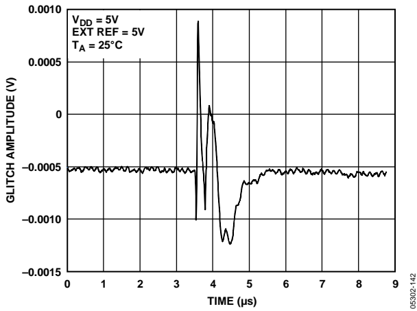
Figure 42. Analog Crosstalk
