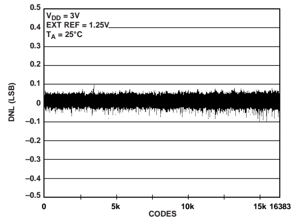
Figure 22. DNL AD5648-1
