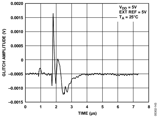
Figure 43. DAC-to-DAC Crosstalk
