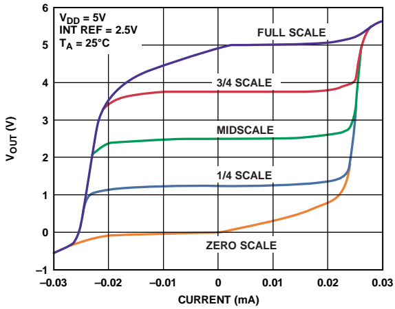
Figure 31. AD5668-2/AD5668-3 Source and Sink Capability
