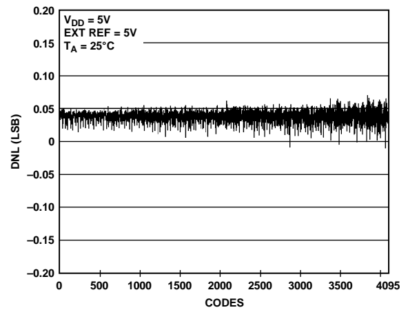
Figure 11. DNL AD5628—External Reference
