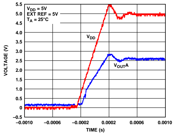
Figure 39. Power-On Reset to Midscale
