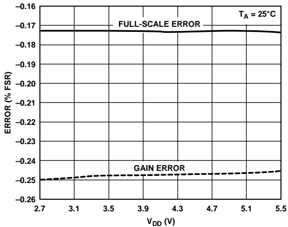
Figure 26. Gain Error and Full-Scale Error vs. Supply Voltage
