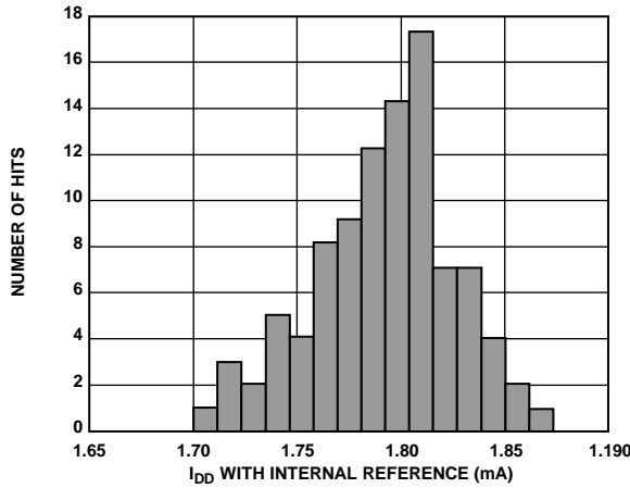
Figure 29. I_{DD} Histogram with Internal Reference
