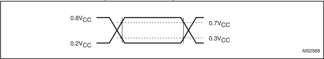
Figure 14. AC testing I/O waveform
