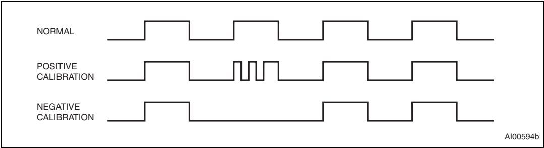
Figure 12. Calibration waveform
