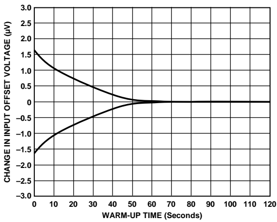
Figure 29. Change in Input Offset Voltage vs. Warm-Up Time
