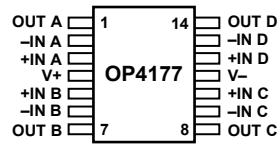
Figure 6. 14-Lead TSSOP (RU Suffix)
