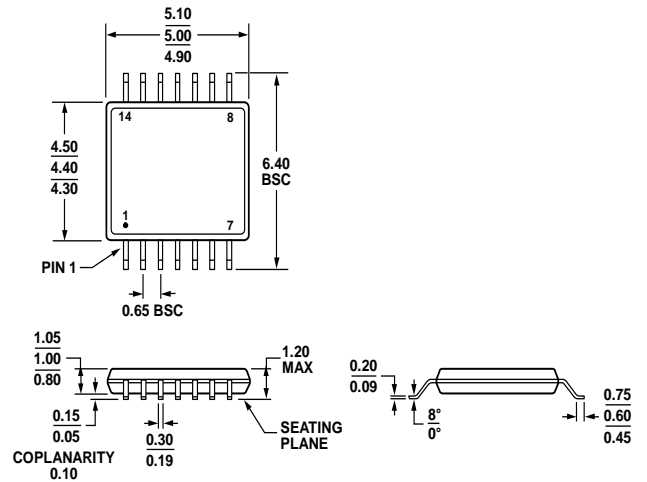
Figure 4. 14-Lead Thin Shrink Small Outline Package [TSSOP] (RU-14) Dimensions shown in millimeters
