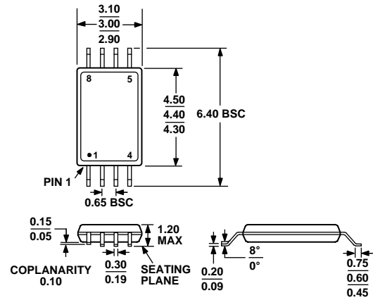
Figure 3. 8-Lead Thin Shrink Small Outline Package [TSSOP] (RU-8) Dimensions shown in millimeters
