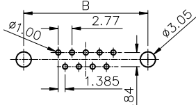
RECOMMEND PCB LAYOUT (TOLERANCE ±0.05)
