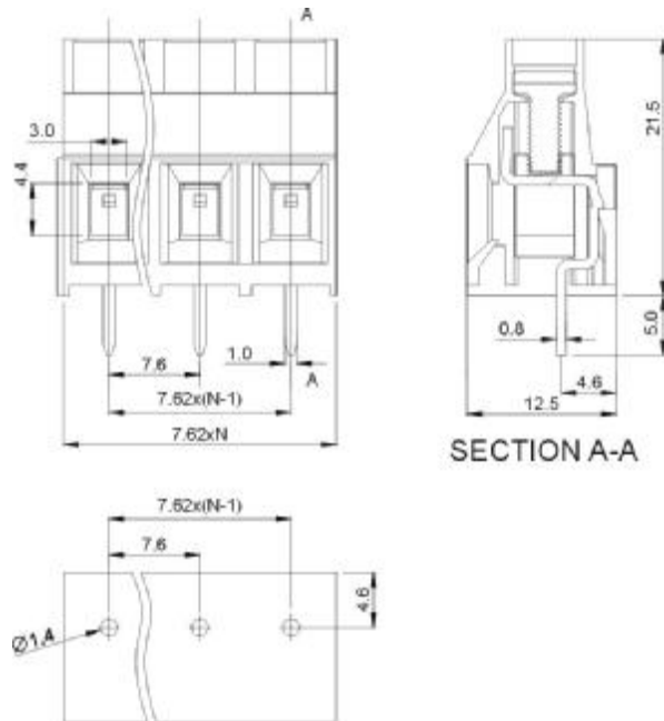
PCB LAYOUT
