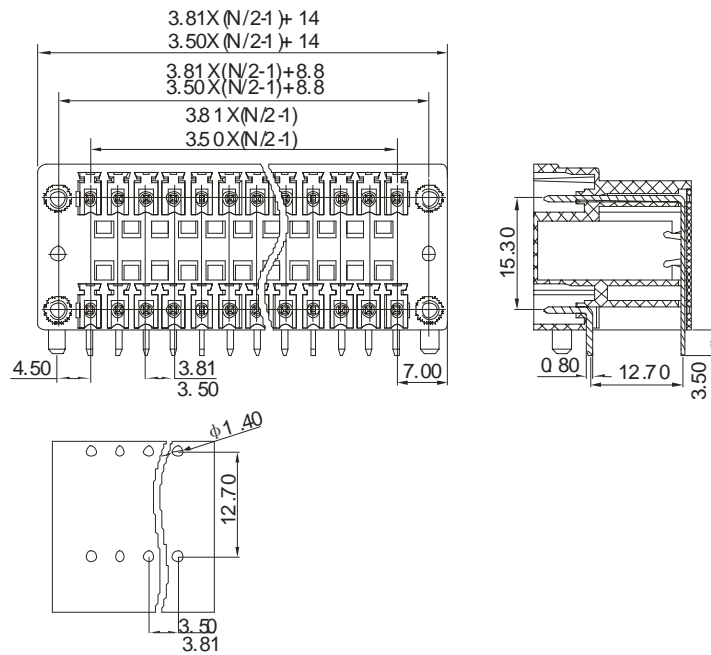
PCB LAYOUT
