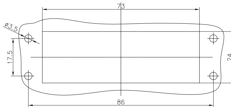
Panel cut out
